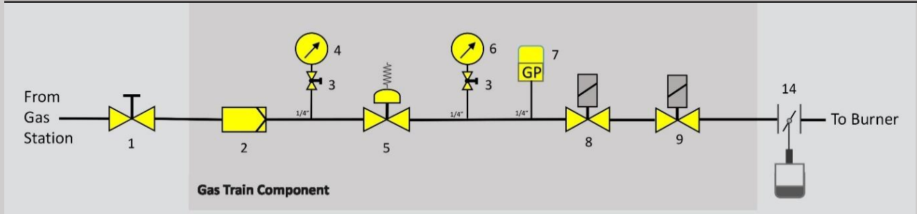
GT1 (Pressure input<500 mbar, separated items)
