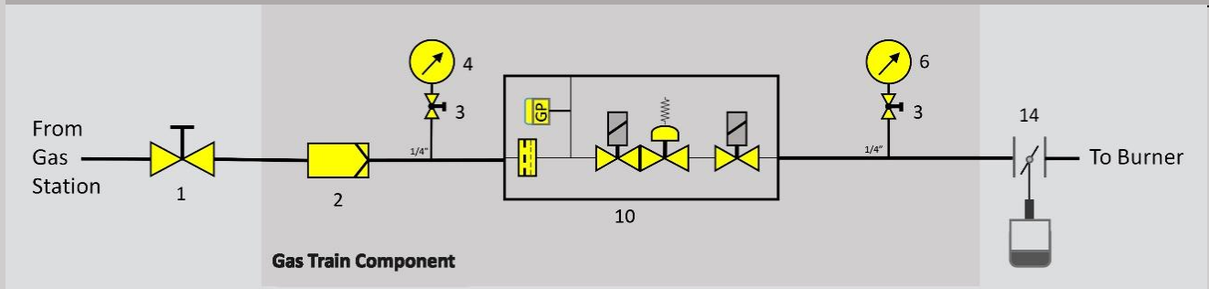
GT2 (Pressure input<500 mbar, multi bloc gas train)
