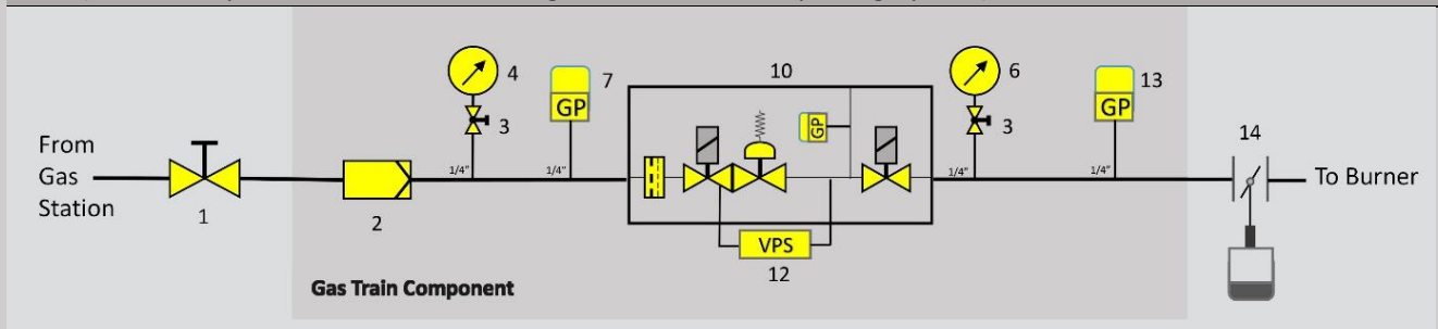
GT4 (Pressure input<500 mbar, multi bloc gas train, with valve proving system)
