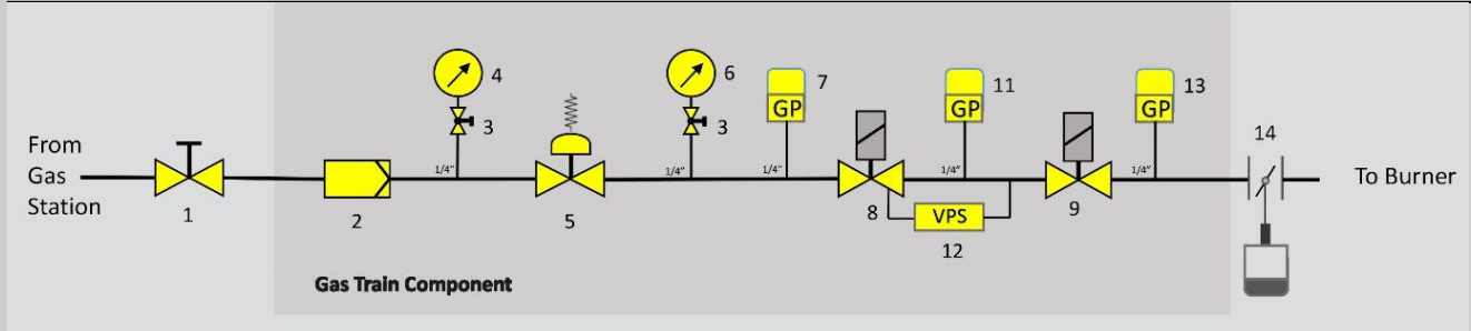
GT3 (Pressure input<500 mbar, separated items,with valve proving system)
